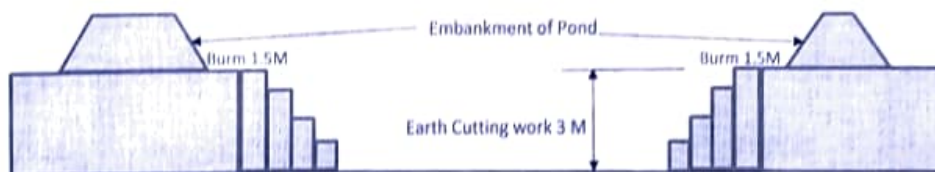
Cross Section of Pond
